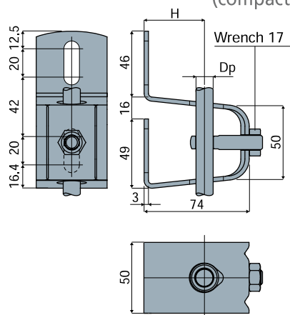
Guide rail bracket (compact version)
