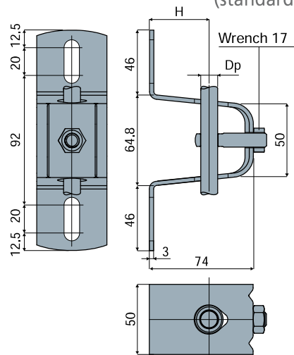
Guide rail bracket (standard version)
